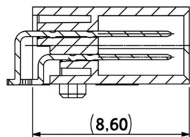
12 Pins
